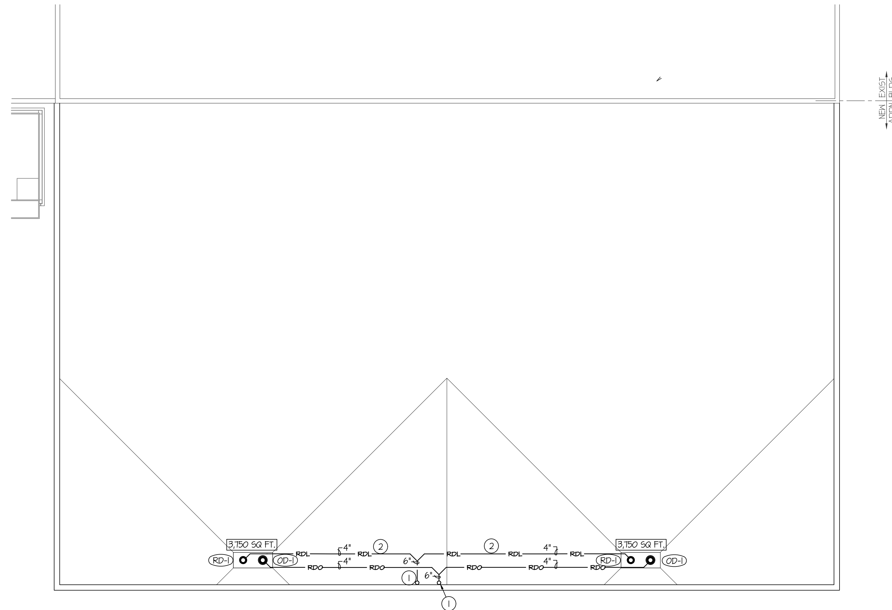
ROOF PLUMBING PLAN SCALE: 1/8" = 1'-0"
